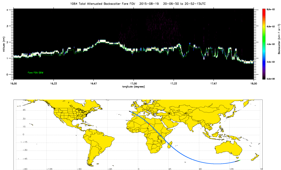
Figure 1. Comparison of the CATS attenuated total backscatter at 1064 (top panel) shows that the surface detected by the instrument (white colors) agrees favorably with the DEM values (green).
