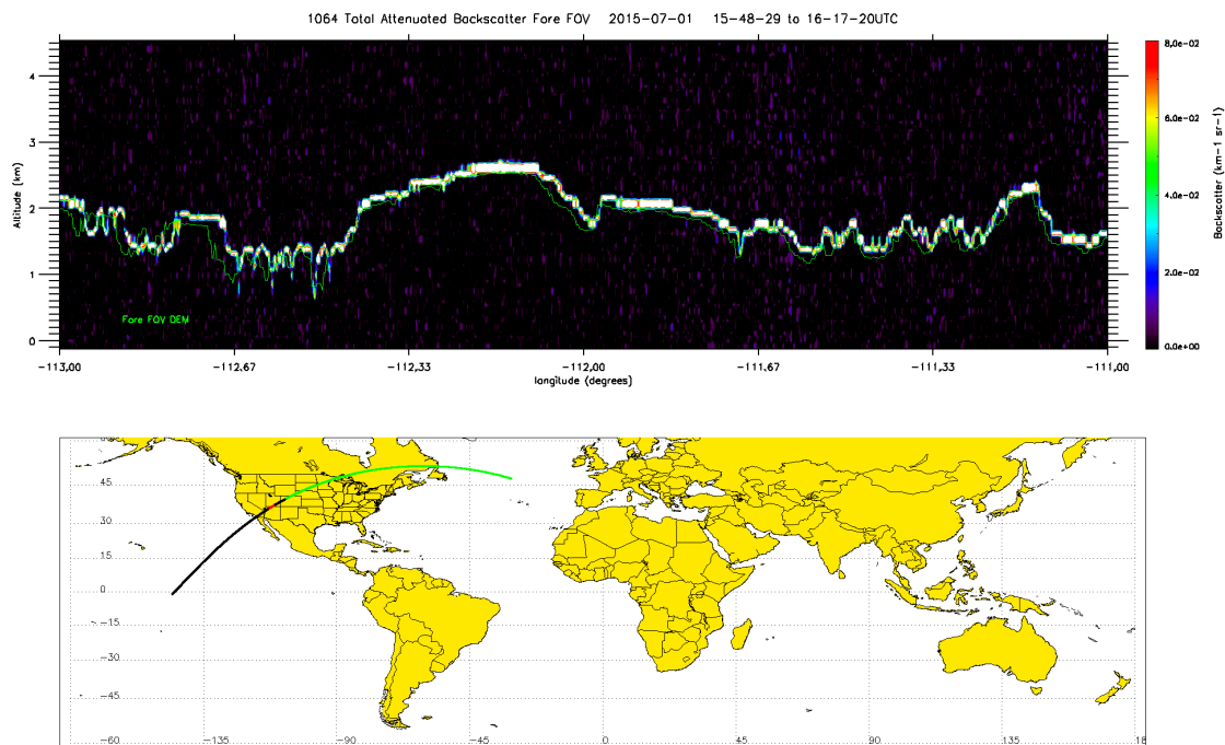
Figure 2. Comparison of CATS attenuated total backscatter at 1064 (top panel) shows that the surface detected by CATS (white colors) is offset slightly along the CATS track compared to DEM values (green).
